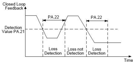
Fig. FA-4 Closed Loop Feedback Loss Detection
