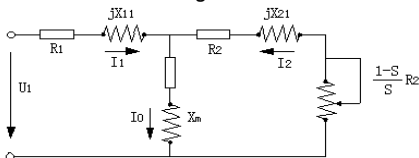
Fig. F2-1 Steady State Equivalent Circuit of Asynchronous Motor
