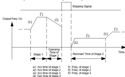
Fig. F9-4 PLC Start Mode 1
