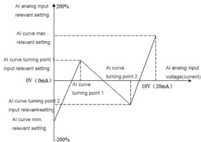
Figure F6-2 AI multi-point curve diagram
