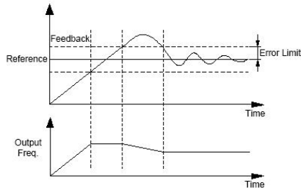
Fig. F8-3 Error Limit Schematic Diagram
