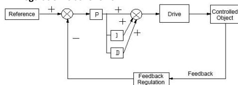
Fig. F8-2 PID Regulation
