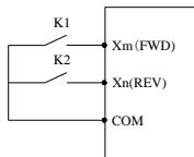
Fig. F7-2 2-wire Control Mode 1
