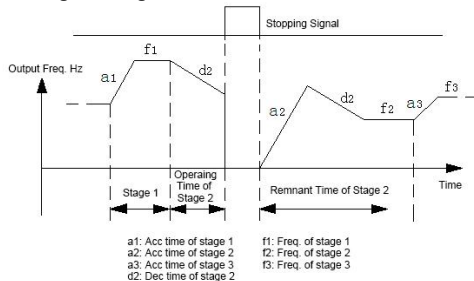
Fig.F9-5 PLC Start Mode 2
