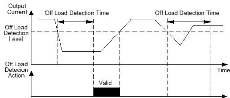
Fig. FA-3 Off Load Detection
