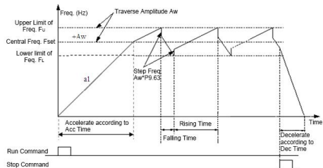
Fig.F9-6 Traverse Operation
