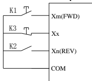
Fig. F7-5 3-wire control mode 2
