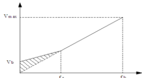
Fig. F5-3 Torque Boost
