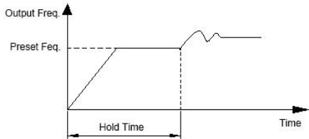
Fig. F8-4 Closed Loop Preset Frequency
