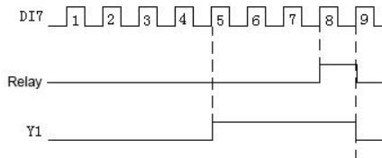
Fig. F7-9 Counter Reset and Detection Setting
