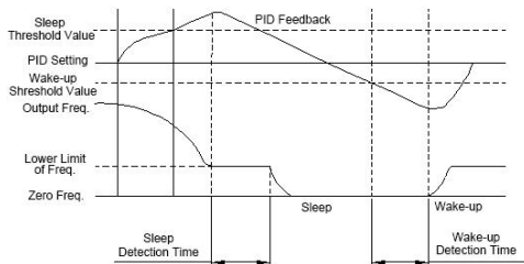
Fig. F8-5 the First Sleep Mode
