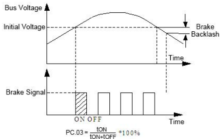
Fig. FC-1 Dynamic Braking
