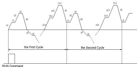
Fig.F9-3 PLC Continuous Cycle
