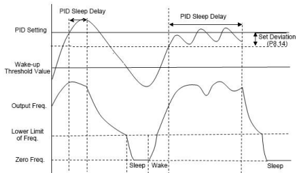
Fig. F8-6 the Second Sleep Mode
