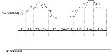
Fig.F9-2 Maintain Last Stage after Single Cycle
