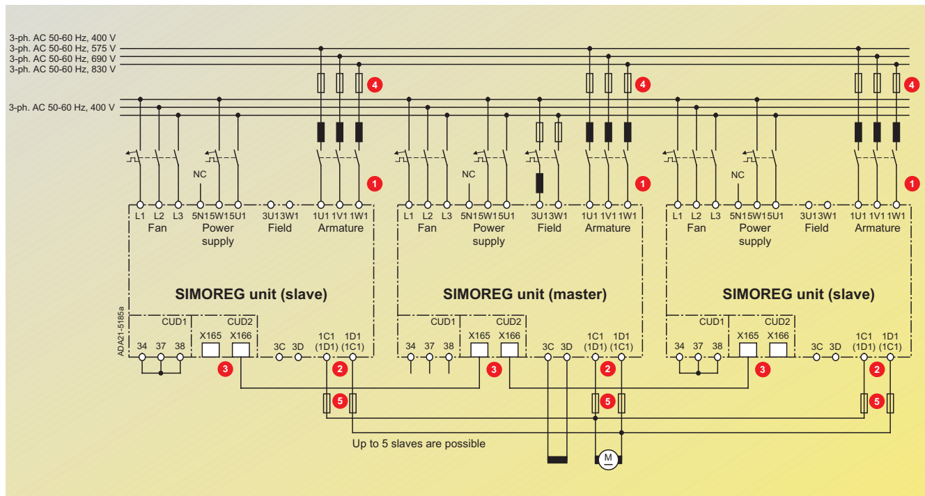
Fig. 5/32 Terminal connections for parallel connection
