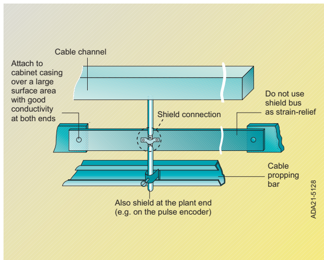
Fig. 5/36 Shielding with routing into the cabinet
