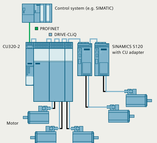
SINAMICS S120 mixed lineup with DRIVE-CLiQ adapter
