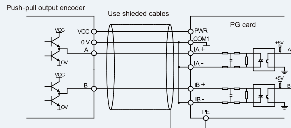
Wiring diagram of push-pull output encoder
