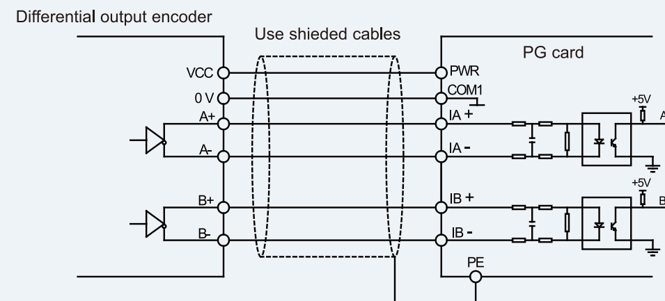
Wiring diagram of open collector output encoder
