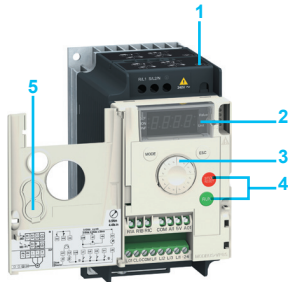
ATV12H075M2 with door on front panel open
