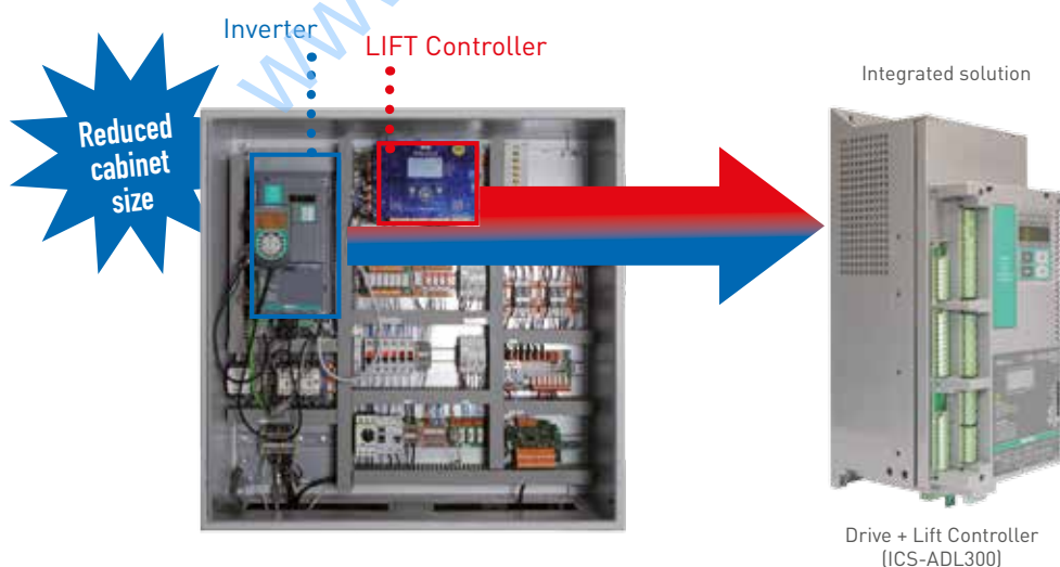
An example of elevator control panel with separate inverter and control card
