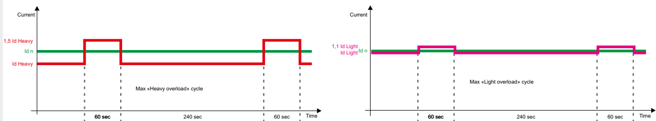
Overload curves
