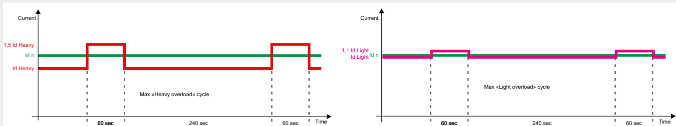
Overload curves
